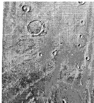
Fig. 1.3 The Chryse Planitia at the Mouth of Ares Vallis. Image Set image #3.
