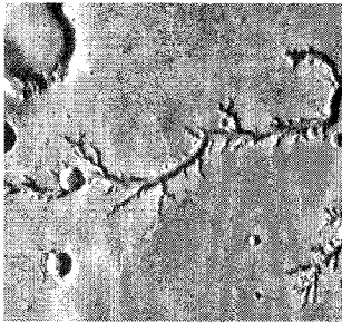
Fig. 7 Nirgil Vallis, an example of a long, winding valley network south of the eastern end of Valles Marineris.
