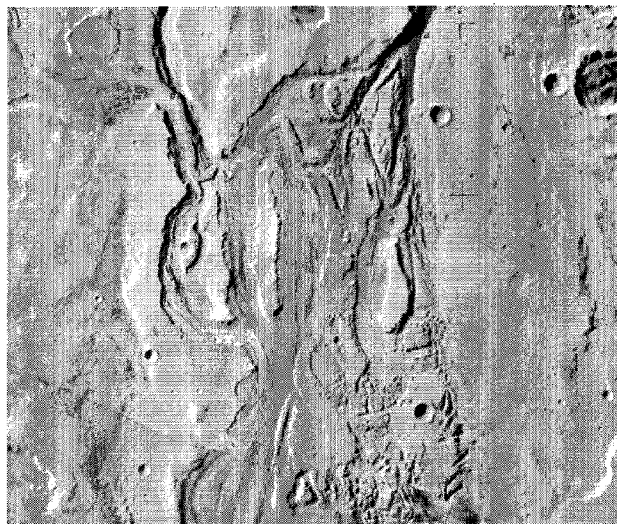
Fig. 5 Source of Mangala Vallis.
