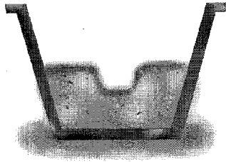
Fig 1.1 Cross-sectional view of the channel in the sand.
