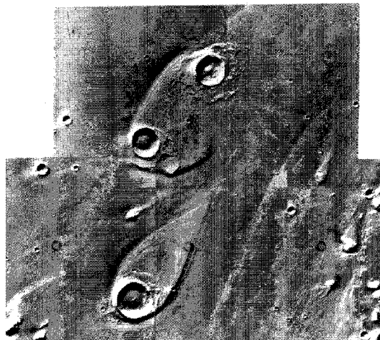
Fig. 4 Eroded Craters at the terminus of the Ares Vallis. Image Set image # 10.
